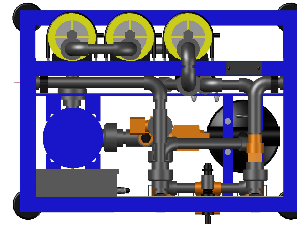
BOMBA GOULDS MOD: 7GBS07 OSMOSIS: 3 MEMBRANAS
